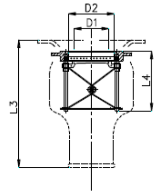
Prise femelle / Push pull series female
